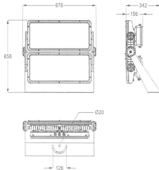
GIANT II 1000W
