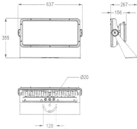
GIANT II 500W
