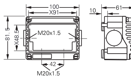
Type 791 01 for metal cable glands
